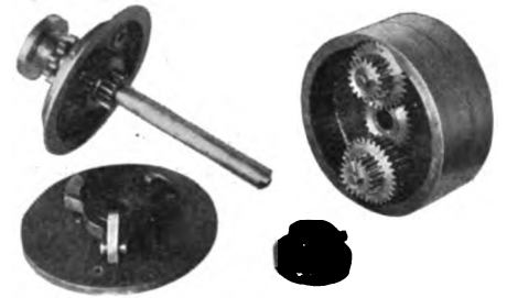
FIG. 3.—PLANETARY GEAR OF MICHIGAN CAR.
